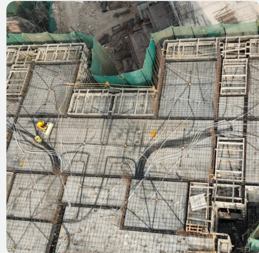
B3 Tower 6th slab completed.
