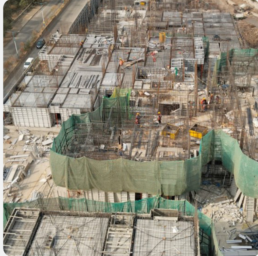
B2 Tower 7th slab completed.
